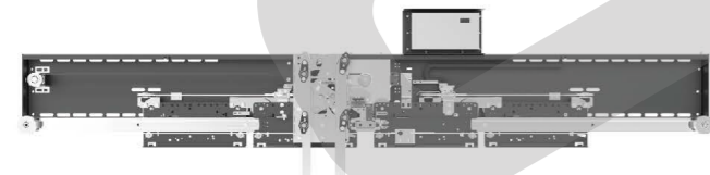
PMA4C-Z 双折中分式门机装置 4-panel center open door operator
