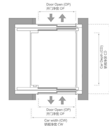
贯通门 Through doors
